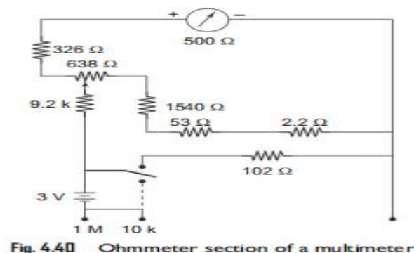
Fig. 4.40 Ohmmeter section of a multimeter
