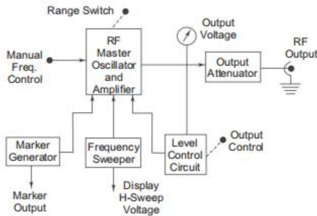
Fig. 8.10 Sweep generator
