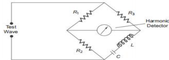
Fig. 9.5 Resonance bridge
