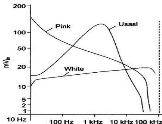
Fig. 8.9 ■ Frequency Response
