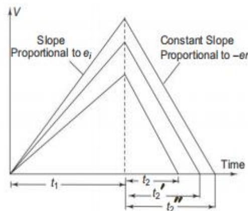
Fig. 5.3 Basic principle of dual slope type DVM
