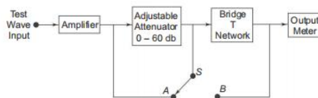
Fig. 9.8 Harmonic distortion analyzer using bridged T-network
